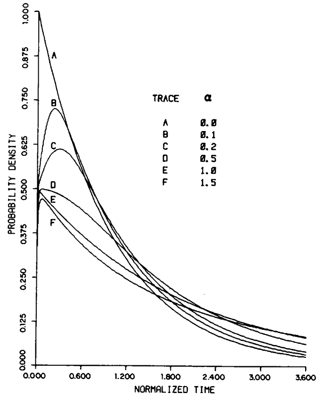
FIGURE 4 Exact solution for the time interval distribution of a damped symmetrical two state random signal. The parameter \alpha is equal to KRC where K is the rate of transitions and RC the time response of the filter. Calculations were carried for K = 1 \text{ s}^{-1} . The normalized time corresponds to K\tau where \tau is the length of the time interval. As seen for normalized times > 1 , the probability density decreases exponentially. This portion of curves can be reproduced using the approximate solution we found for the time interval distribution of a two-state signal (Eq. 23).
