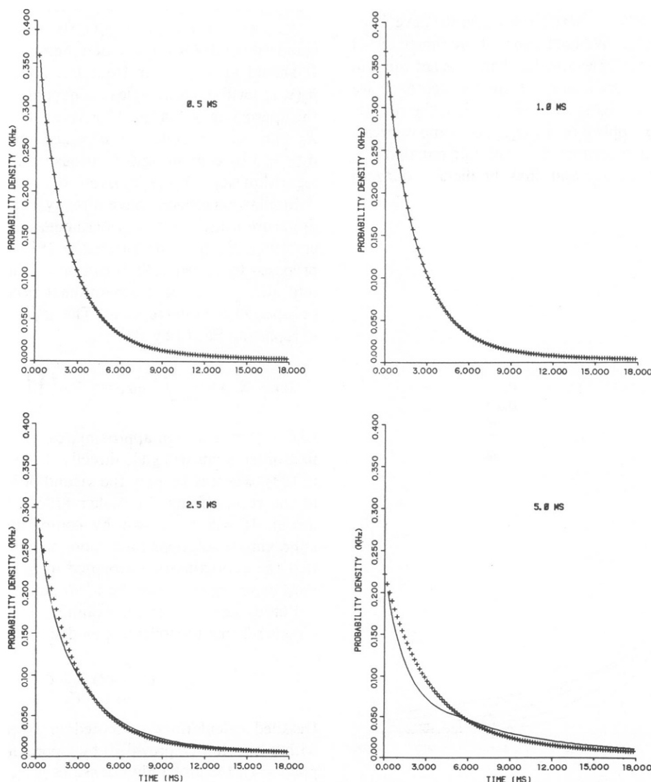
FIGURE 3 Comparison between the exact (continuous line) and approximate (discontinuous line) solution for the closed time interval distribution p_c(\tau, \tau_m) for the three-state model C-O-C. The value of p_c(\tau, \tau_m) was computed using Eq. 16a in one case and Eq. 26b in the other. The value of K_1 , K_2 , K_3 , and K_4 were equal to 75, 25, 100, and 500 s^{-1} , respectively. The value of \tau_m was varied from 0 to 5 ms. Both solutions were found to be equivalent for values of \tau_m smaller than 2 ms.
